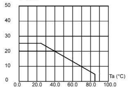
Max forward DC current vs ambient temperature (Tjmax=105°C)
